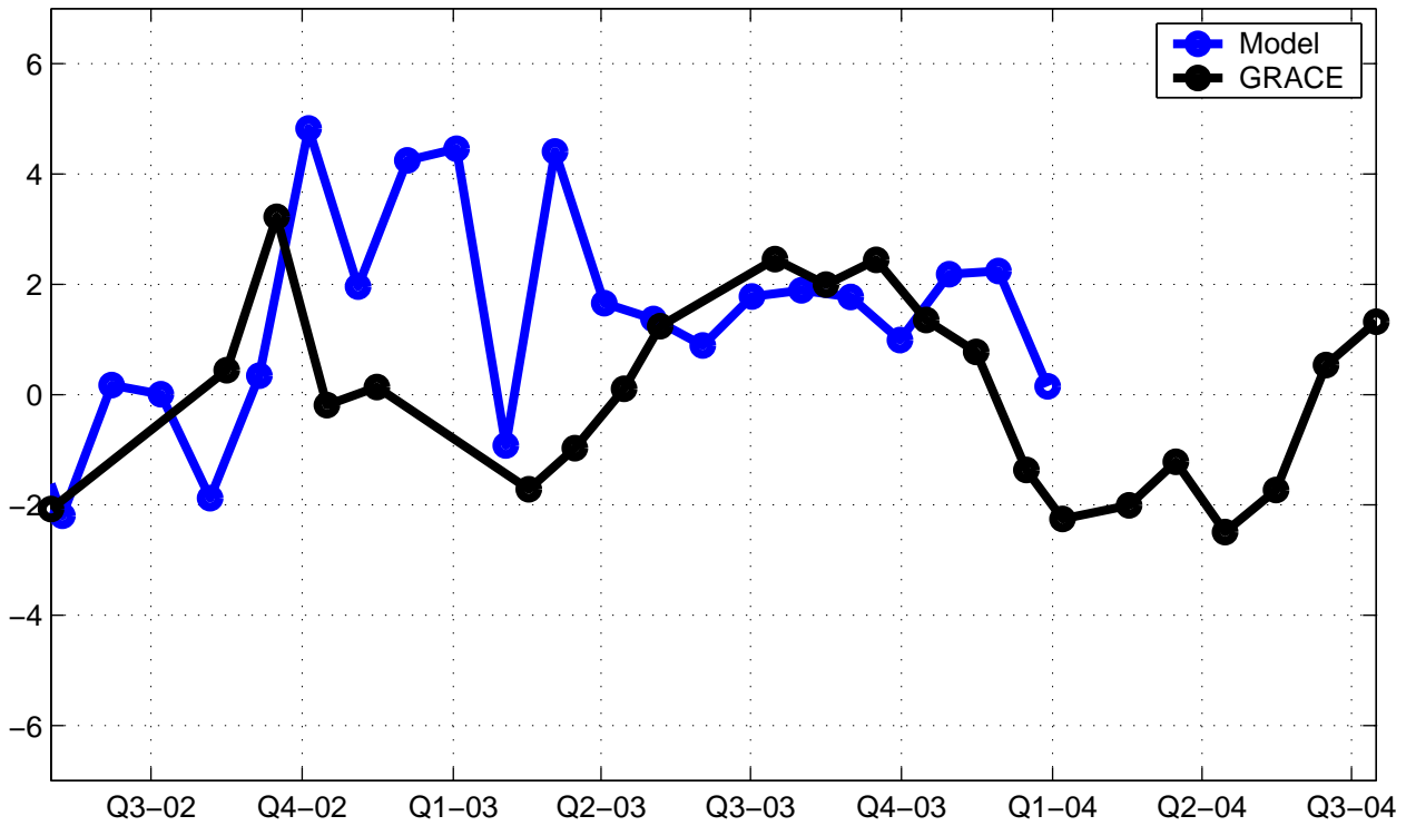
Arctic mass change relative to global ocean (cm)
