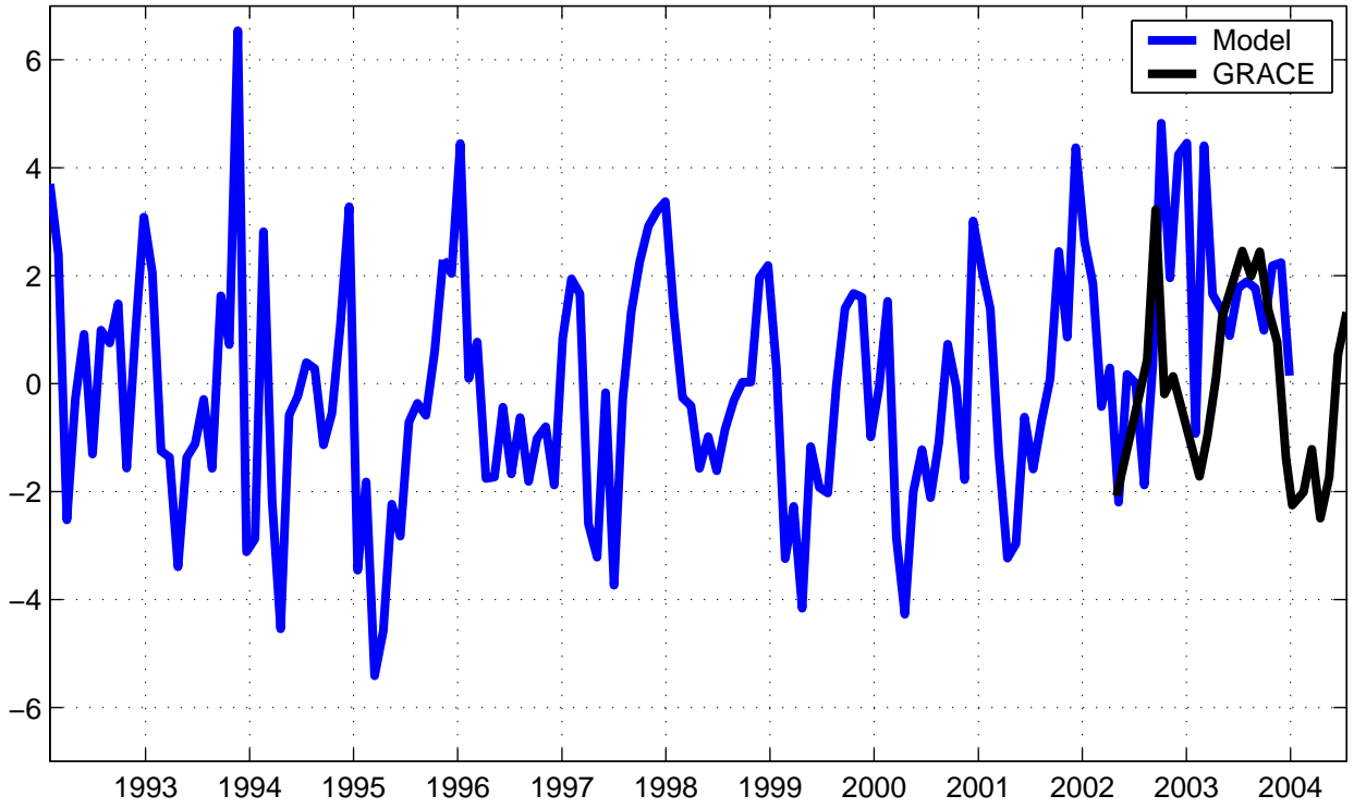
Arctic mass change relative to global ocean (cm)
